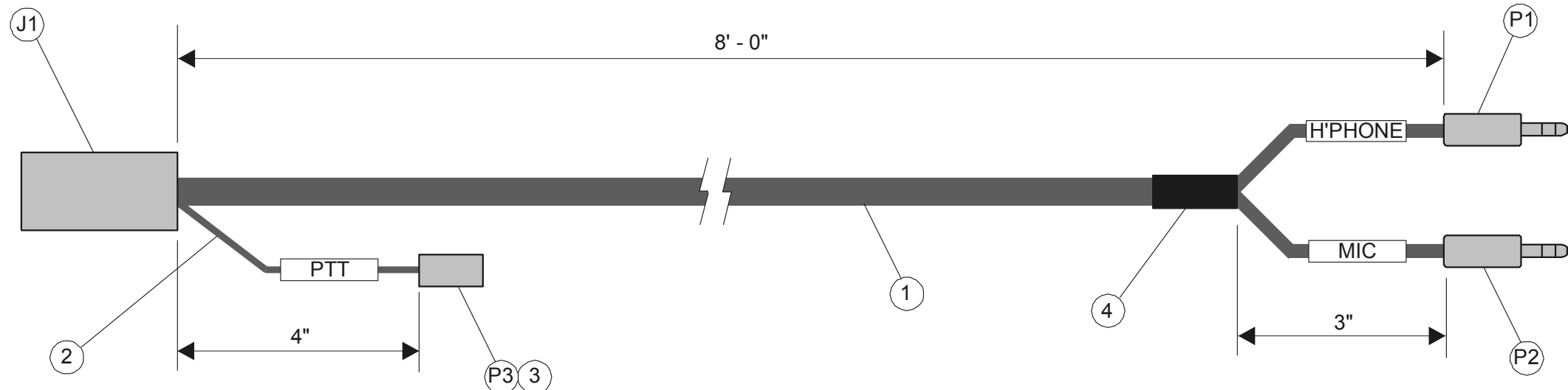
ASSEMBLY DIAGRAM
